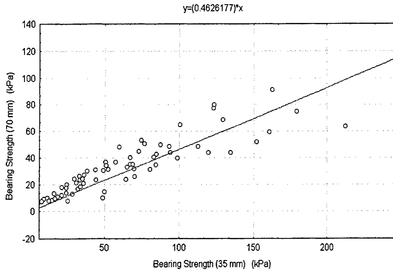
Figure 6. Regression line between bearing strength values obtained with 70 mm flat tip versus those obtained with a 35 mm tip. (Regression coefficient) 2 = 0.712.
