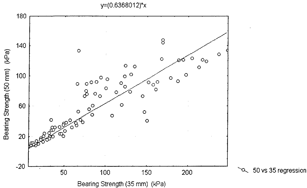
Figure 5. Regression line between bearing strength values obtained with 50 mm flat tip versus those obtained with a 35 mm tip. (Regression coefficient) 2 = 0.746.
