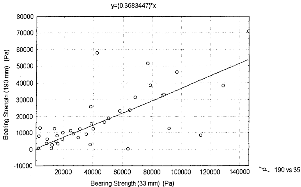
Figure 9. Regression line between bearing strength values obtained with the 190 mm AUSSI penetrometer versus those obtained with a 33 mm diameter ESP penetrometer. (Regression coefficient) 2 = 0.524.
