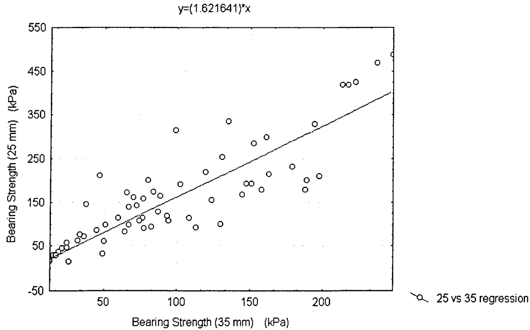
Figure 4. Regression line between bearing strength values obtained with 25 mm flat tip versus those obtained with a 35 mm tip. (Regression coefficient) 2 = 0.731.
