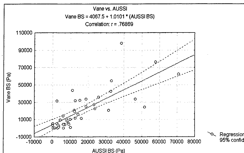
Figure 11. Linear regression between bearing strength values from vane-shear device and AUSSI (from Mulhearn et al., 1999). (\text{Regression coefficient})^2 = 0.59 .
