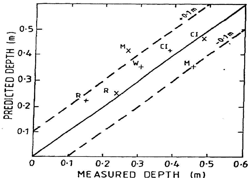
Figure 12. Comparison of predicted versus measured mine burial depth from Mulhearn (1993). Predictions were based on sediment shear strength data obtained with a vane-shear device.
