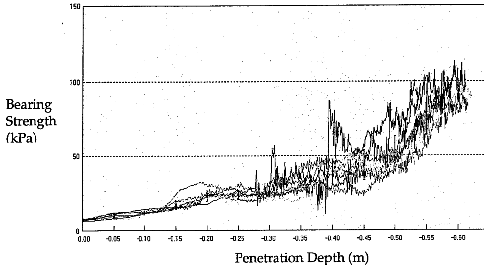
Figure 3. Frame grab from STING software of analysed impacts at station 5, 6 September 2001.
