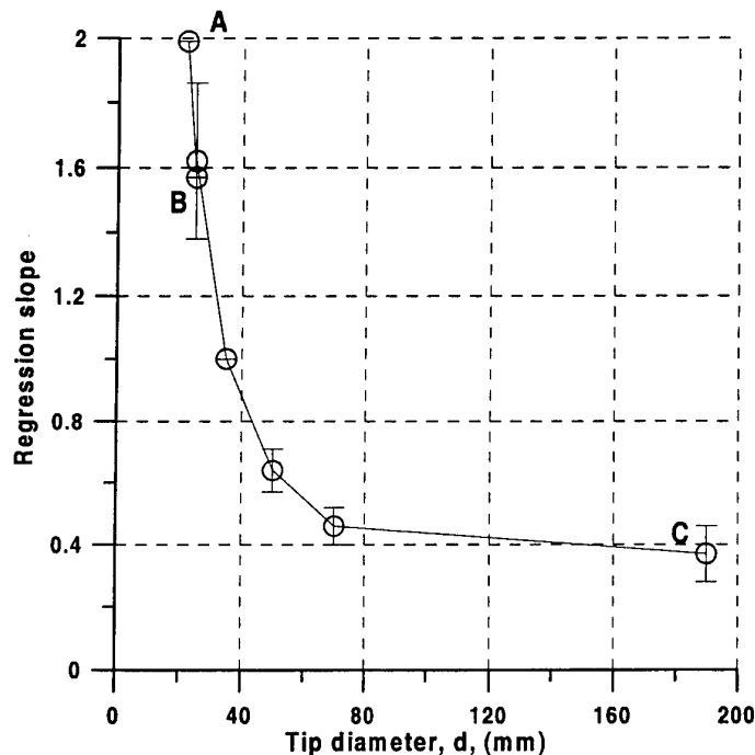
Figure 10. Slope of regression line versus penetrometer tip diameter. Point labelled A is for 22mm ESP versus 33 mm ESP. Point labelled B is for 25 mm STING versus 33 mm ESP. Point labelled C is for AUSSI versus 33 mm ESP. Other points are for various STINGs of diameter, d , versus 35 mm STING. (Error bars, where shown, show 95% confidence limits for regression slope values)
