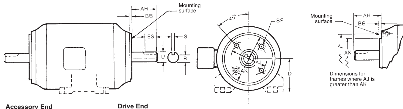
Accessory End
